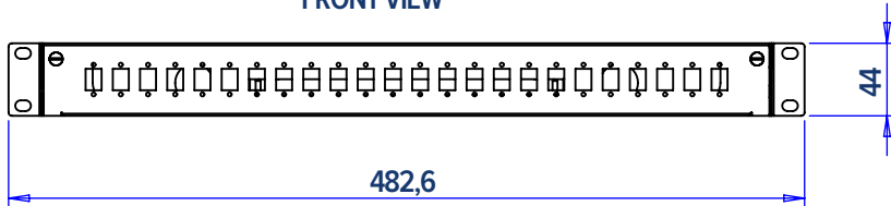
FRONT VIEW
