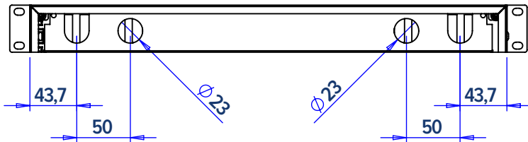
REAR VIEW
